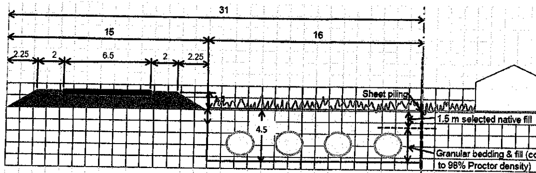
Figure 3.3 Transmission line – Intake to Dhaka-Sylhet Highway Junction
