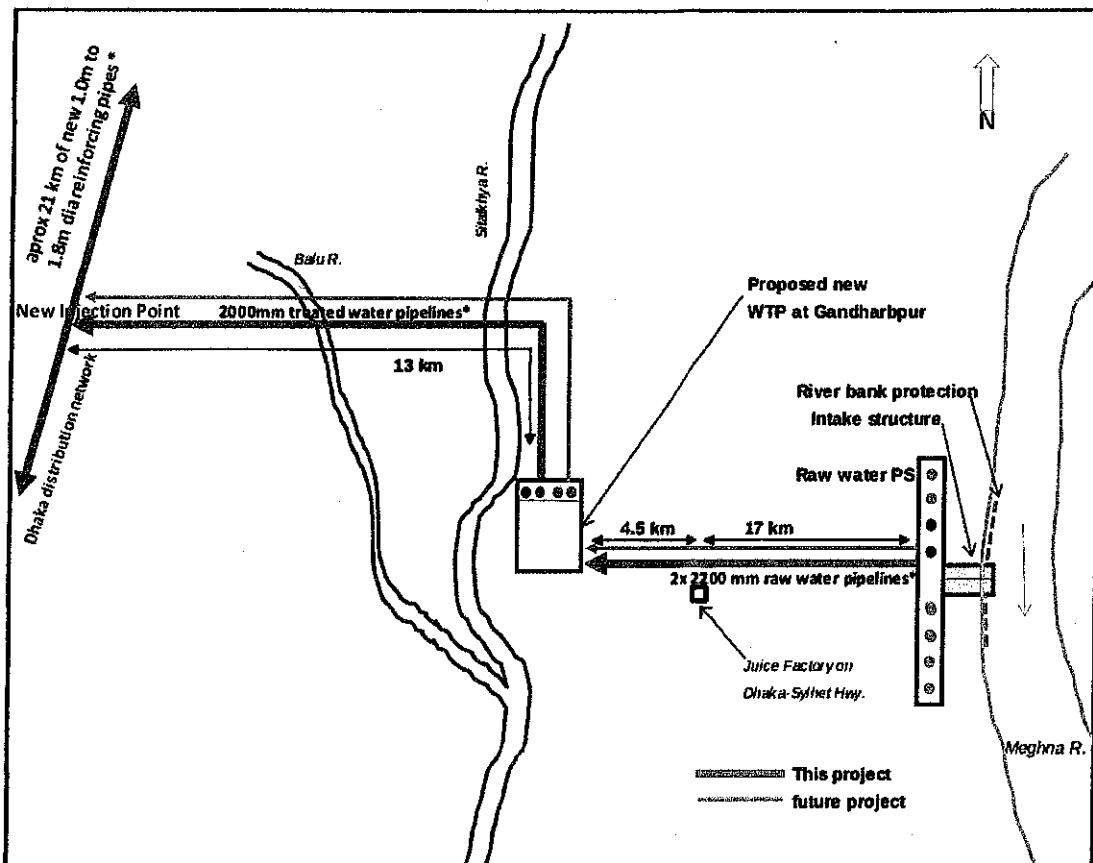
Figure 3.2: Schematic Project Layout Plan
