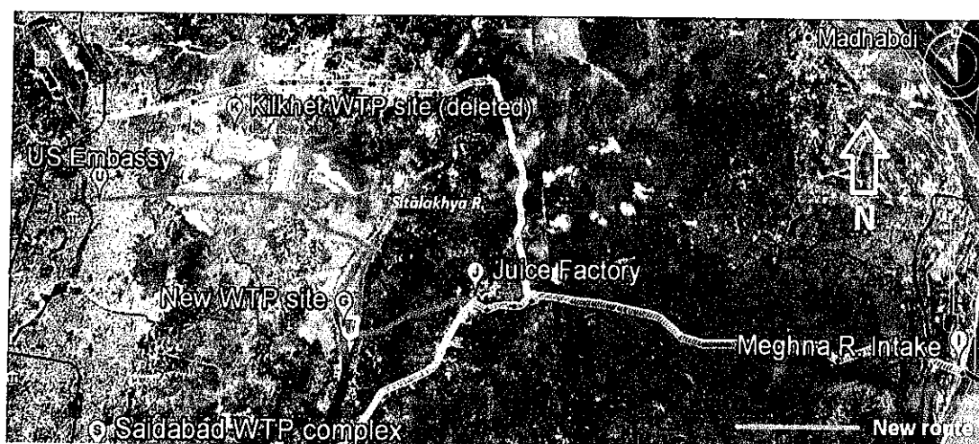
Figure 3.1: Project Lay-out Plan
